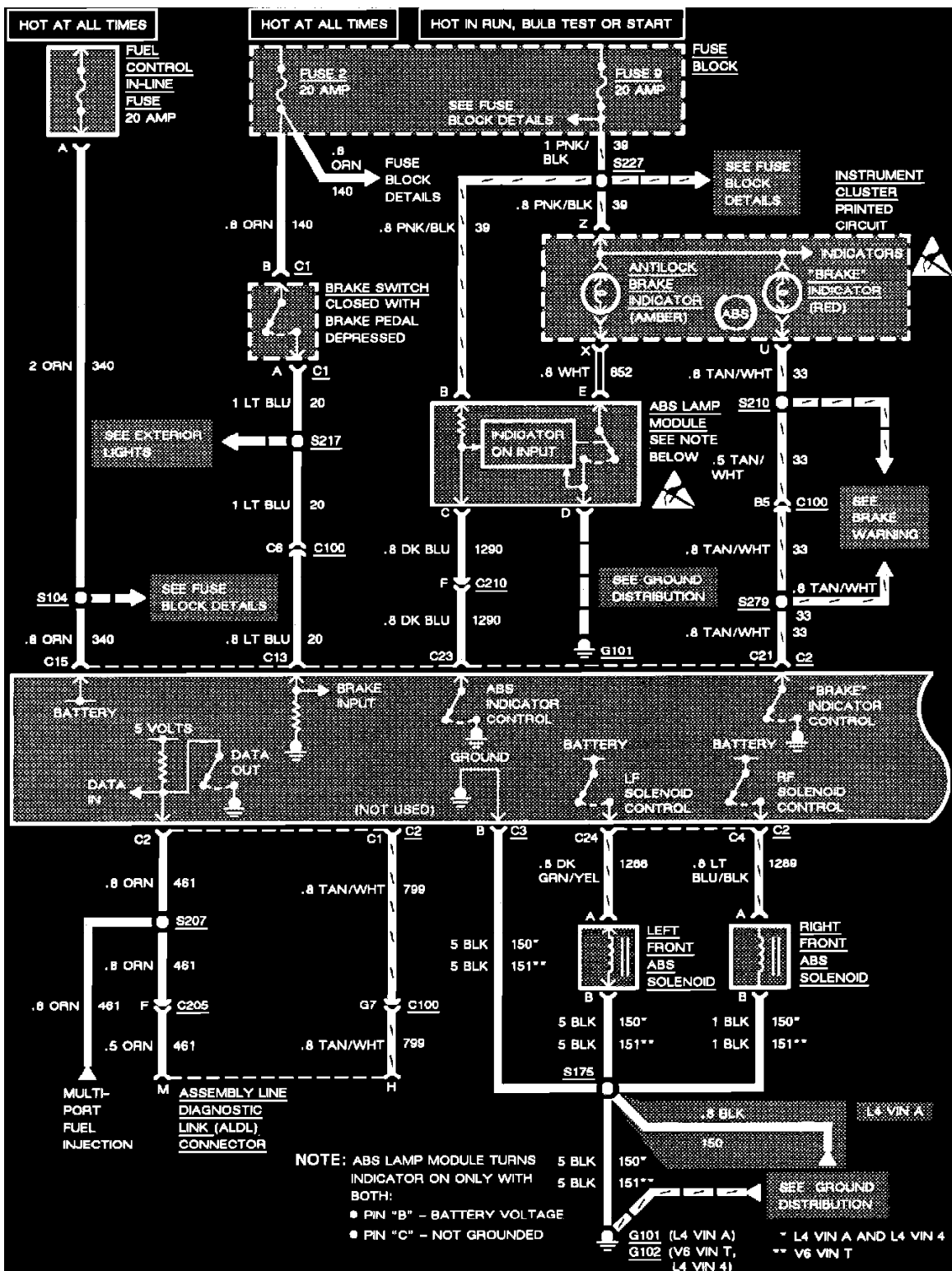
Antilock Brake System
